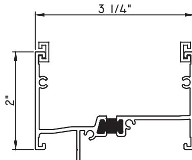
2" STACK MULL M17032 - STACK MULL M6270 - C-MULL (QTY. 2) 72406 - END DAM (QTY. 2) BRBTT46 - POP RIVET (QTY. 8) 970-300 - WEEP COVER
