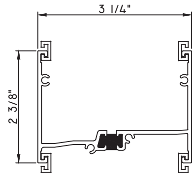
2 3/8" STACK MULL M22015 - STACK MULL M6270 - C-MULL (QTY. 2 OR 4) QWP-032917 - END DAM (QTY. 2) BRBTT46 - POP RIVET (QTY. 8) 970-300 - WEEP COVER
