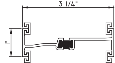
1" STACK MULL M21087 - STACK MULL M6270 - C-MULL (QTY. 2 OR 4) 970-300 - WEEP COVER
