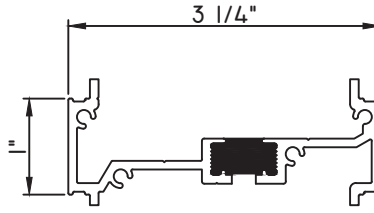
1" STACK MULL M23723 - STACK MULL 970-300 - WEEP COVER QWP-M23846 - END DAM (QTY. 2) QWP-M23845 - END DAM (QTY. 2) BRBTT46 - POP RIVET (QTY. 8)
