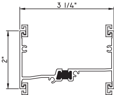
2" STACK MULL M16318 - STACK MULL M6270 - C-MULL (QTY. 2 OR 4) 72406 - END DAM (QTY. 2) BRBTT46 - POP RIVET (QTY. 8) 970-300 - WEEP COVER
