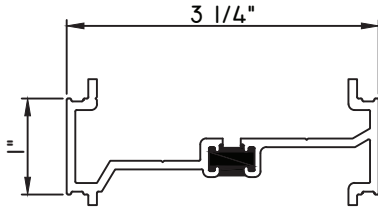
1" STACK MULL M537248 - STACK MULL 970-300 - WEEP COVER
